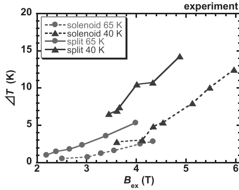
Fig. 3. Temperature rise \Delta T measured on the side of the sample holder as a function of the applied field B_{\text{ex}} for the solenoid- and split-coils.
