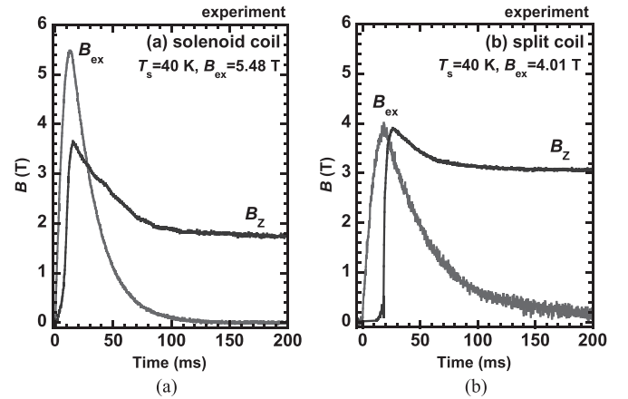
Fig. 5. Time dependence of the local field B_Z(t) at the center of the bulk surface for each coil, (a) solenoid coil and (b) split coil, after applying the optimum applied field B_{\text{ex}}^* .
