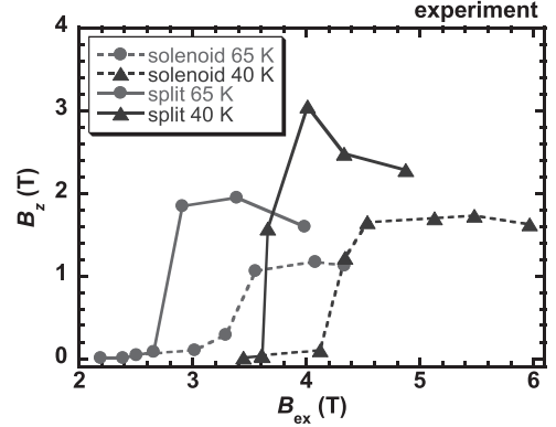
Fig. 2. Experimental results of the trapped field B_z at the center of the bulk as a function of the applied field B_{ex} using the solenoid- and split- coils at 65 K and 40 K.
