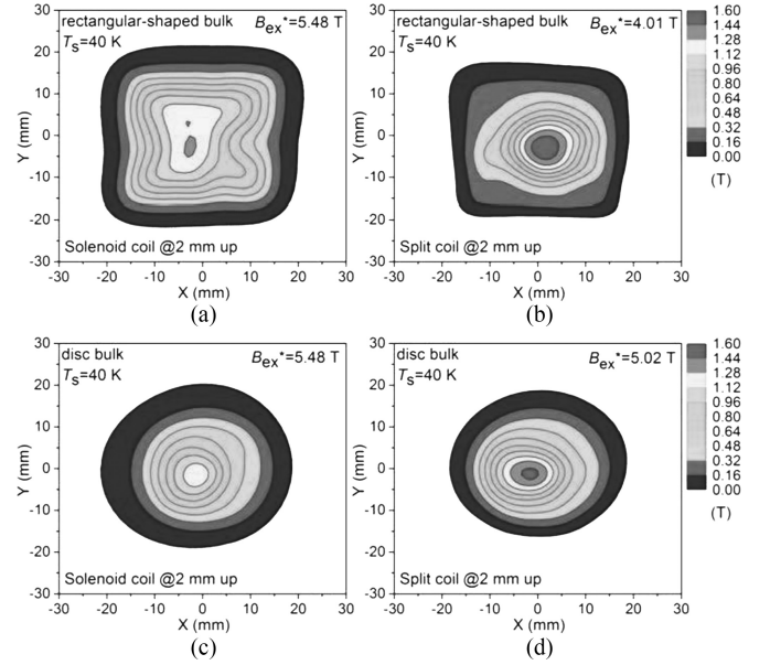
Fig. 4. Experimental results of the trapped field profiles measured at 2 mm above when full magnetization for the rectangular-shaped bulk, using (a) the solenoid- and (b) split- coils and for the disc bulk using (c) the solenoid- and (d) split- coils reported by M. D. Ainslie et al. [11] at 40 K.
