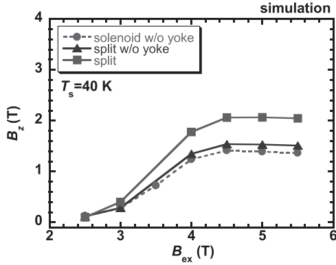
Fig. 6. Analysis results of the trapped field B_Z at the center of the bulk as a function of the applied field B_{ex} for each coil.
