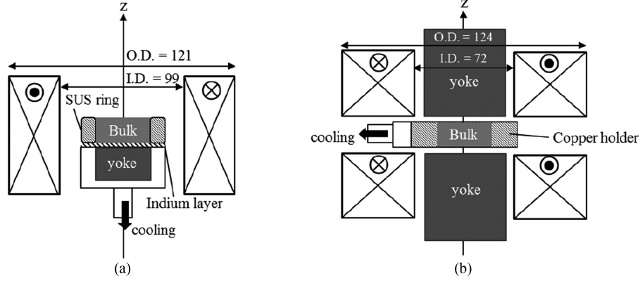
Fig. 1. Experimental setup of two kinds of apparatus for PFM and the magnetizing coil, (a) solenoid-type and (b) split-type.
